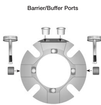
S20 Streamline Dual Seal
