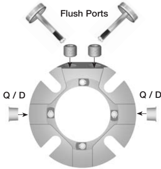
S10 Streamline Single Seal
